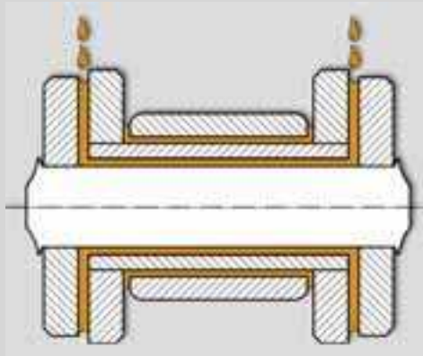
Fig. 2: Cross-section of a chain link
